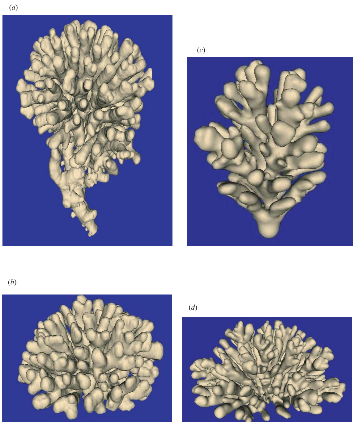
Figure 1. Surface-renderings of CT scans of Madracis mirabilis colonies and simulated objects. C indicates the compactness. (a) Upward-growing morphology ( C = 0.29 ) and (b) hemispherical morphology ( C = 0.41 ) of M. mirabilis . Simulated growth forms: (c) upward-growing morphology ( C = 0.30 ) and (d) hemispherical morphology ( C = 0.24 ). Animations of all objects shown in figure 1 can be found in electronic Appendix B.
