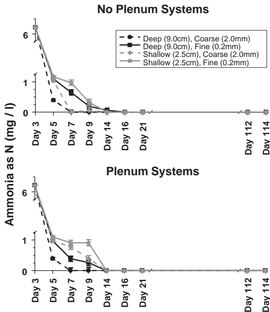
Fig. 2. Time series plot of the mean ammonium ( \text{NH}_4^+ as N) concentration (mg/l) in experimental aquaria.
