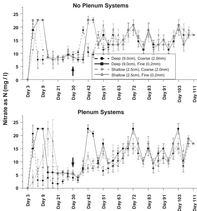
Fig. 4. Time series plot of the mean nitrate as N ( \text{NO}_3^- as N) concentration (mg/l) in experimental aquaria. Arrows designate the start of continuous dosing of ammonium (see text).
